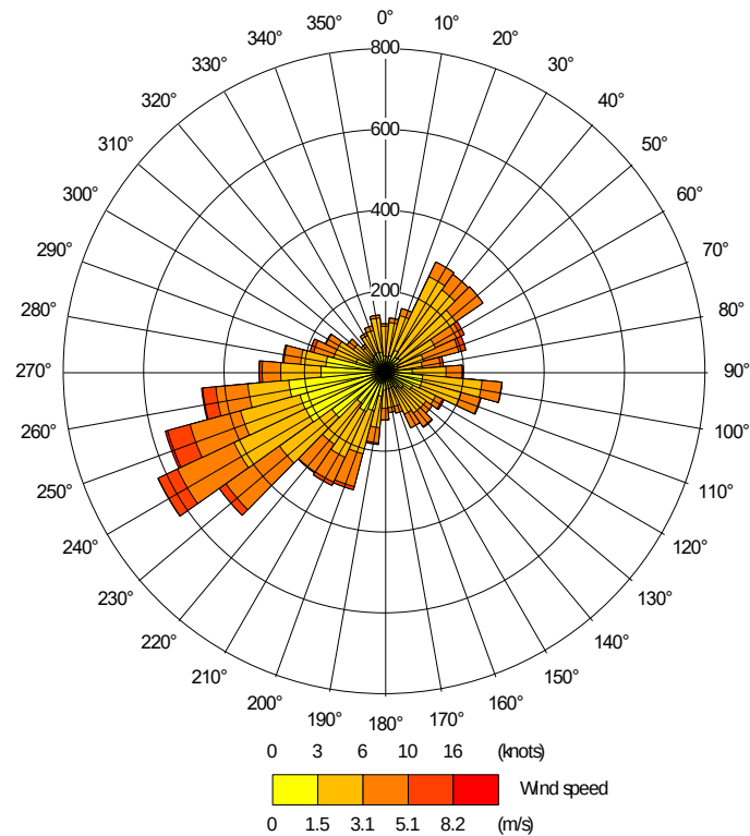
Figure 3: Wind Rose from Cippenham Meteorological Station for 2018
