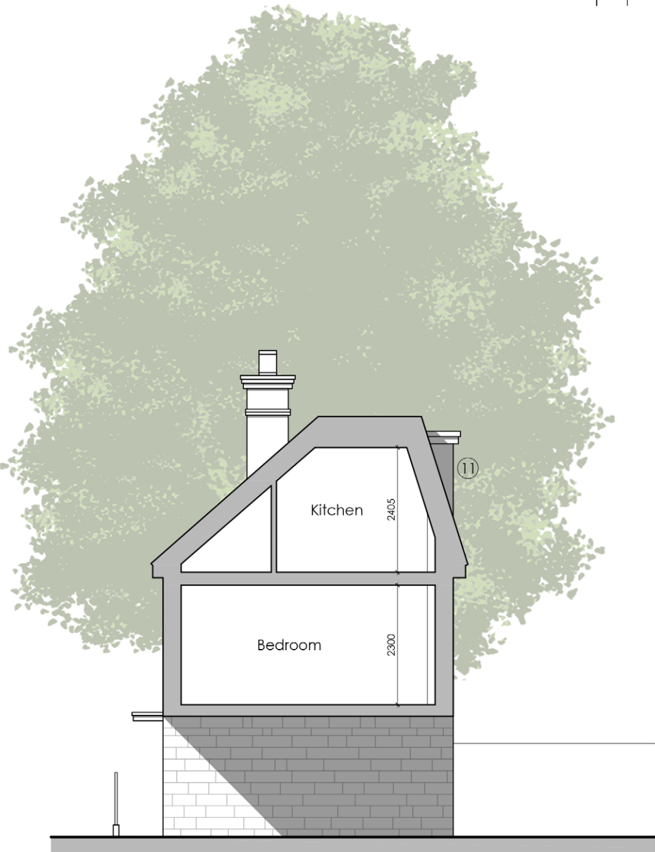
PREVIOUS APPROVAL SECTION AA 1:100
