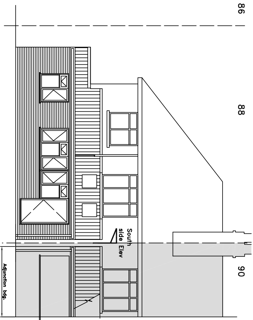
REAR ELEVATION PROPOSED and also indicating adjunction building
