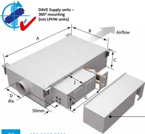
SUPPLY FAN SIZE DS1 - DATA LPHW 82/71 (Deg C)
