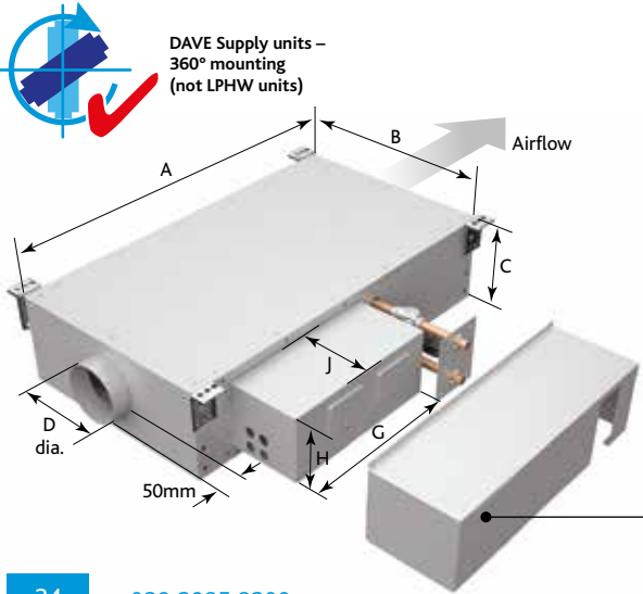
SUPPLY FAN SIZE DS2H - DATA LPHW 82/71 (Deg C)
