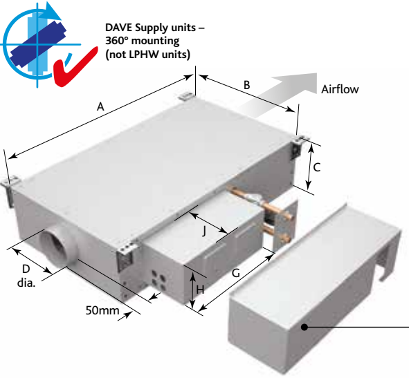
SUPPLY FAN SIZE DS3 - DATA LPHW 82/71 (Deg C)
