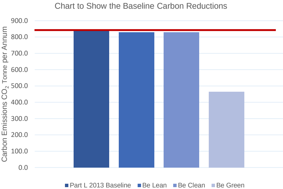
Chart 6.1 A chart to show the baseline carbon emissions of the proposed building
