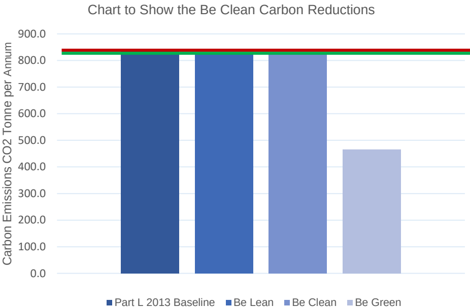
Chart 6.3 A chart to show the Be Clean carbon emissions reductions of the proposed building
