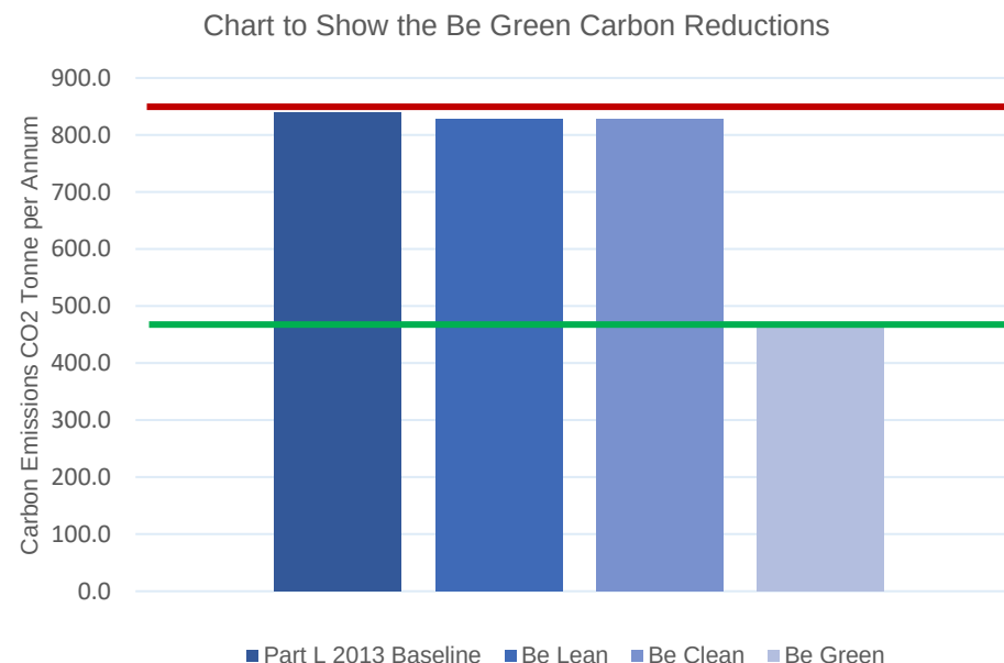
Chart 6.4 A chart to show the Be Green carbon emissions reductions of the proposed building
