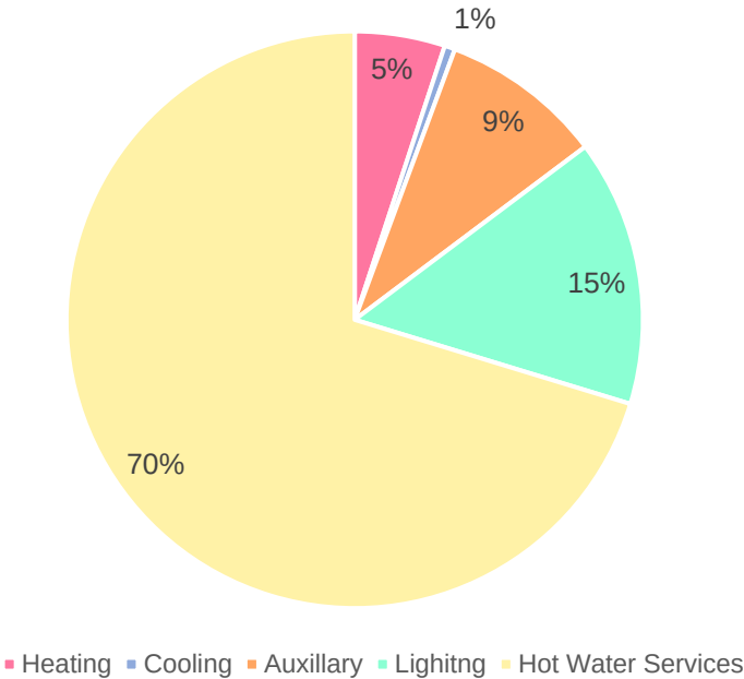
Predicted Building Energy Rates (kWh.m -2 )
