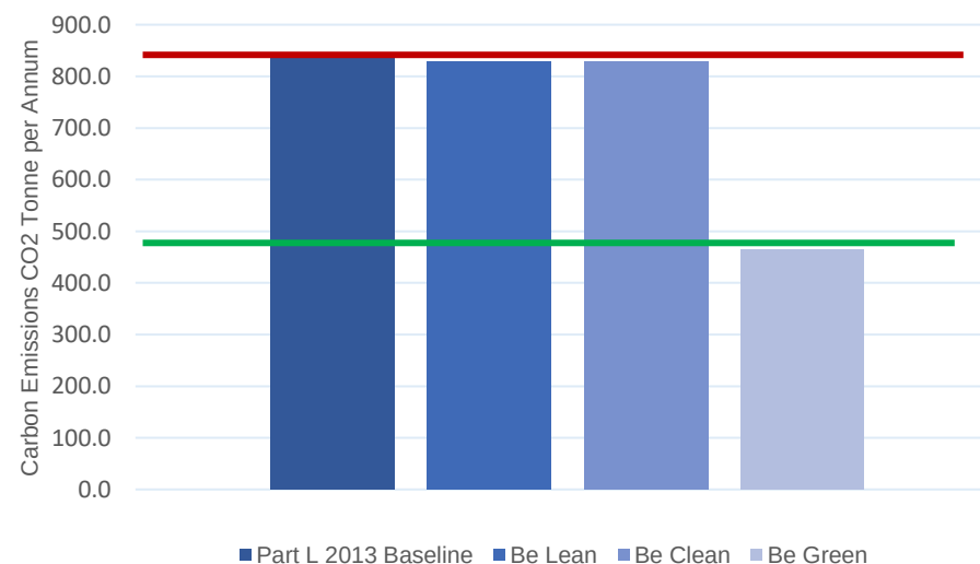
Chart to Show the Be Green Carbon Reductions
