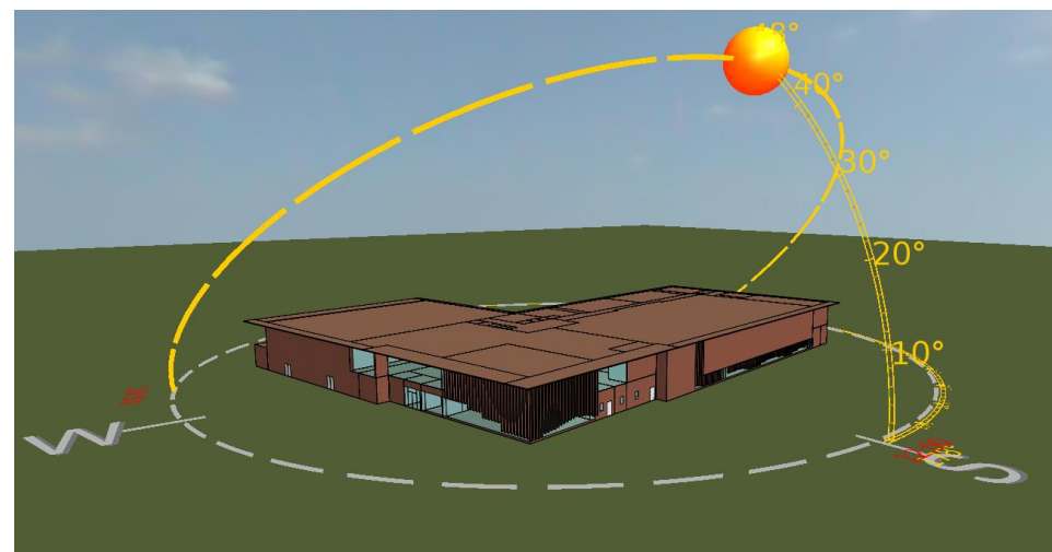
Figure 2.0 Image to show the orientation of the building in energy modelling software IES VE
