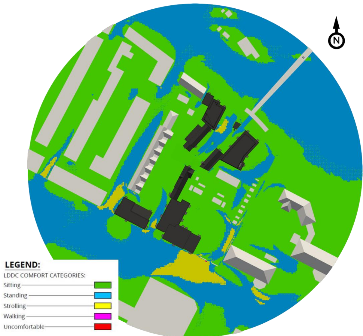
Figure 19: Configuration 3 – Proposed Development with the Cumulative Surrounding Buildings – Ground and Podium Level, Autumn Season
