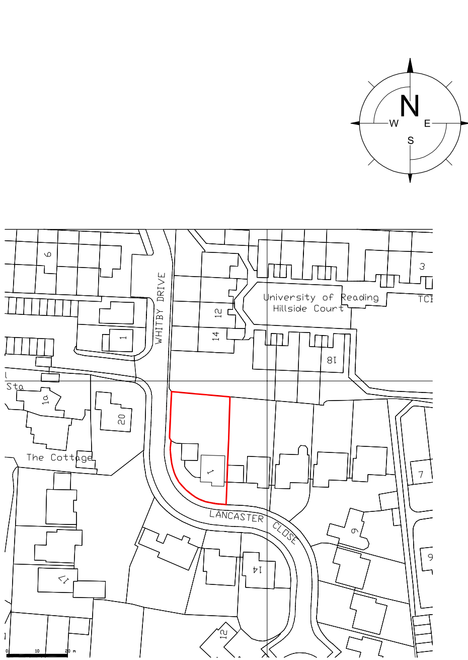
Location Plan (1:1250)
