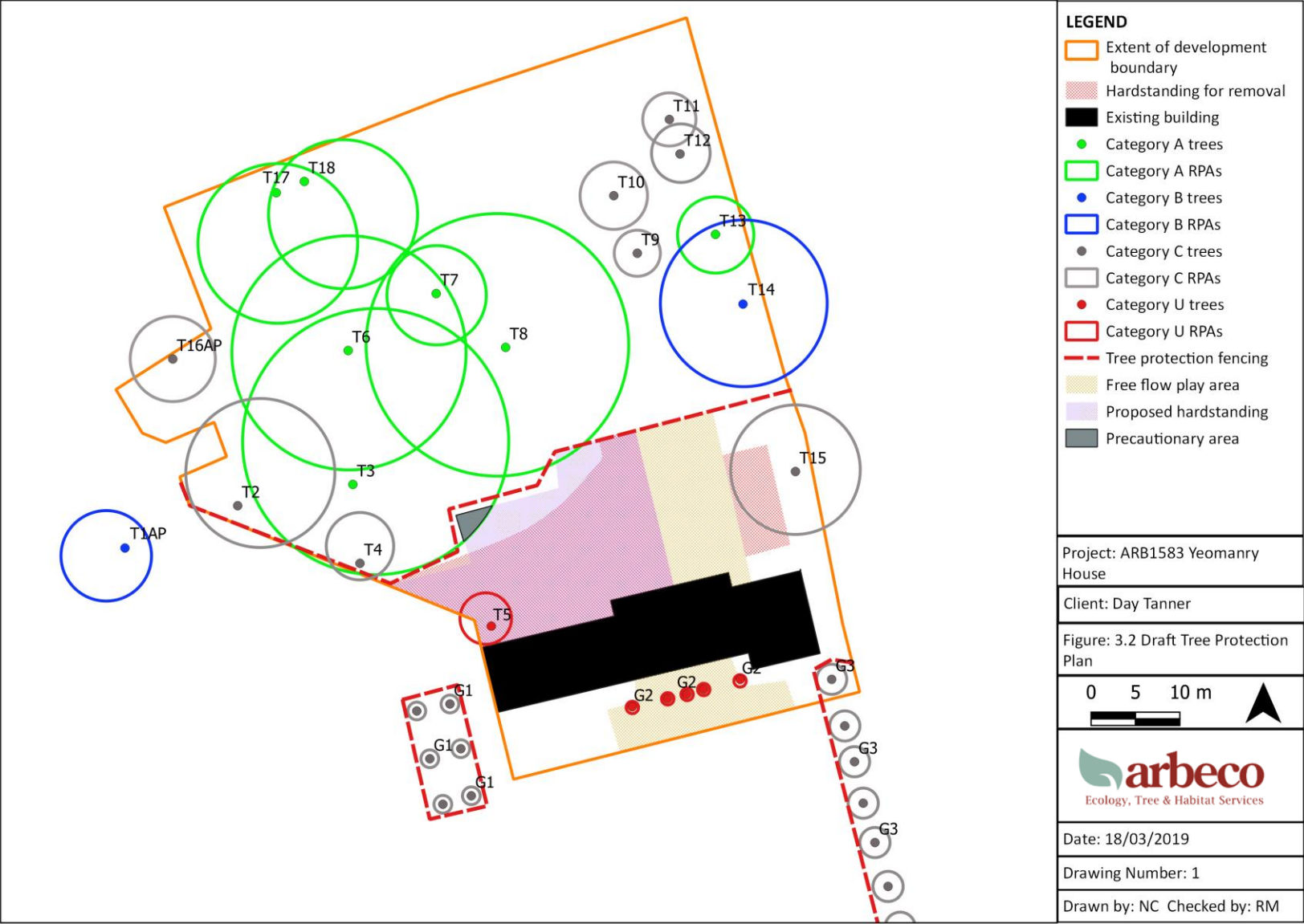
Figure 3.2: Tree Protection Plan
