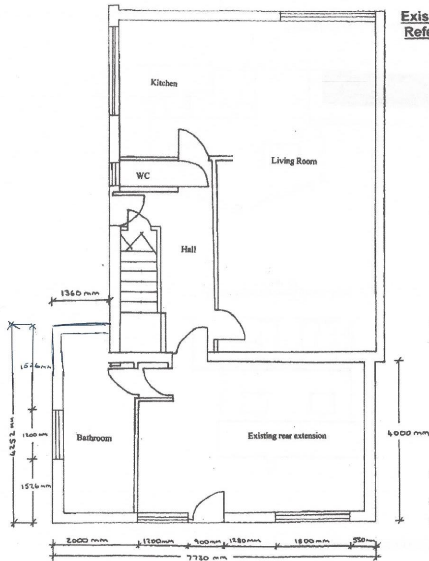
Existing ground floor – Ref: B1
