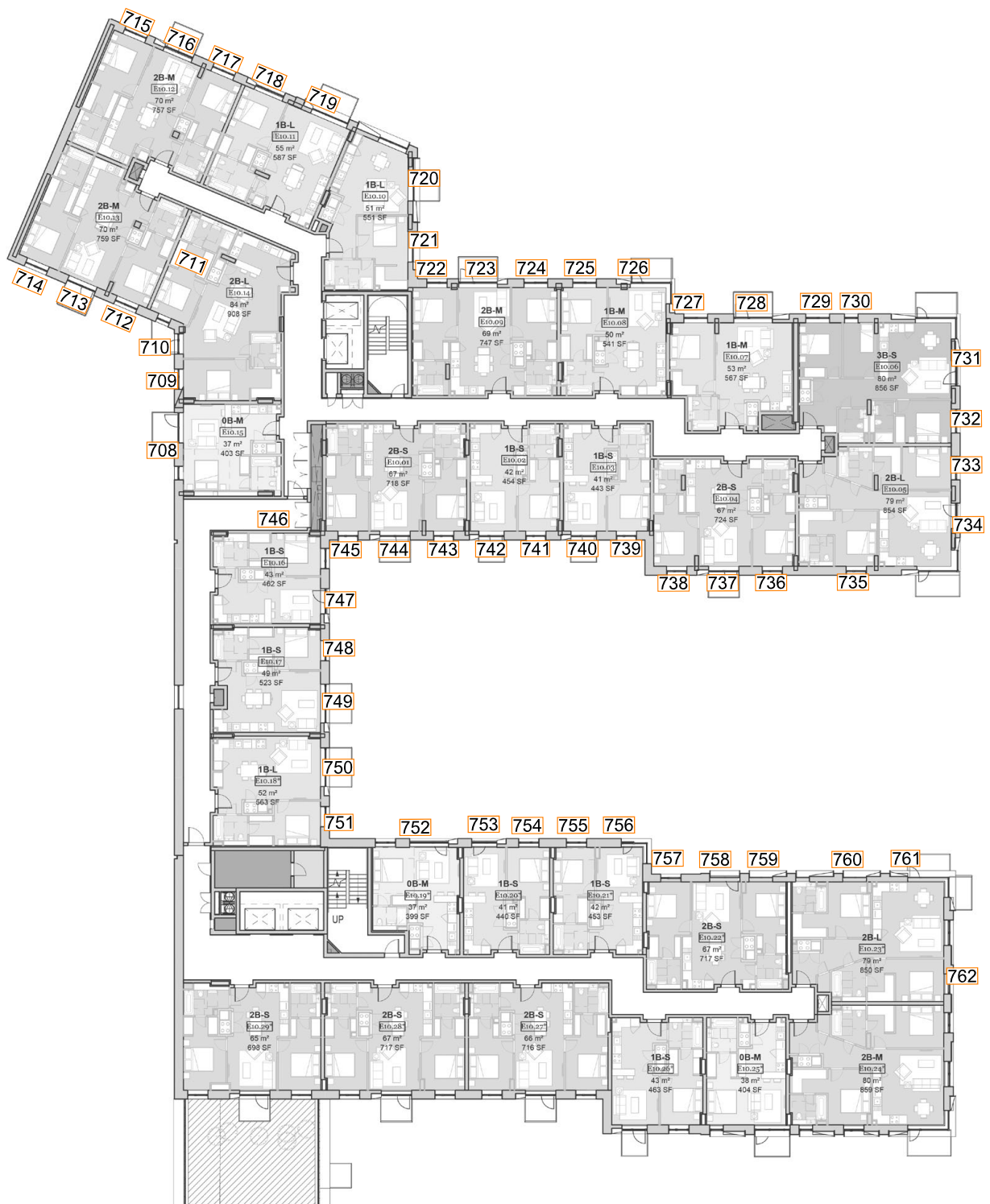
Fig. 21: Floor Plan
