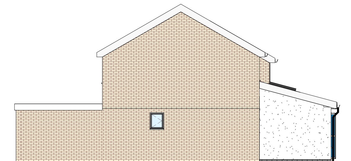
Proposed Right 1 : 100
