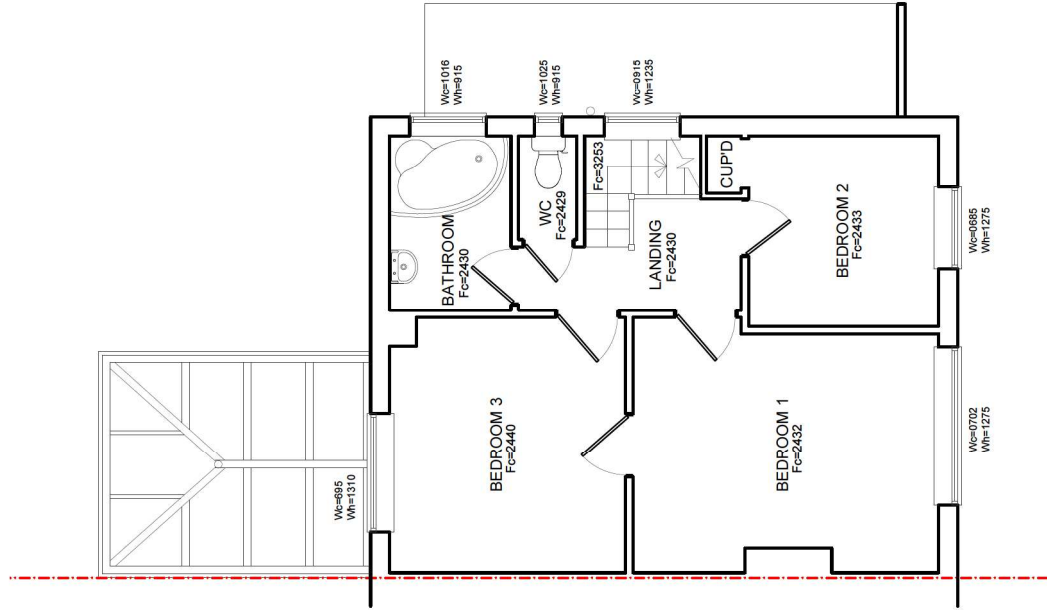
First Floor 1:100
