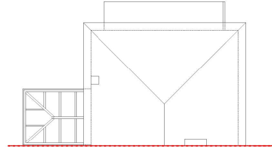
Roof Plan 1:200
