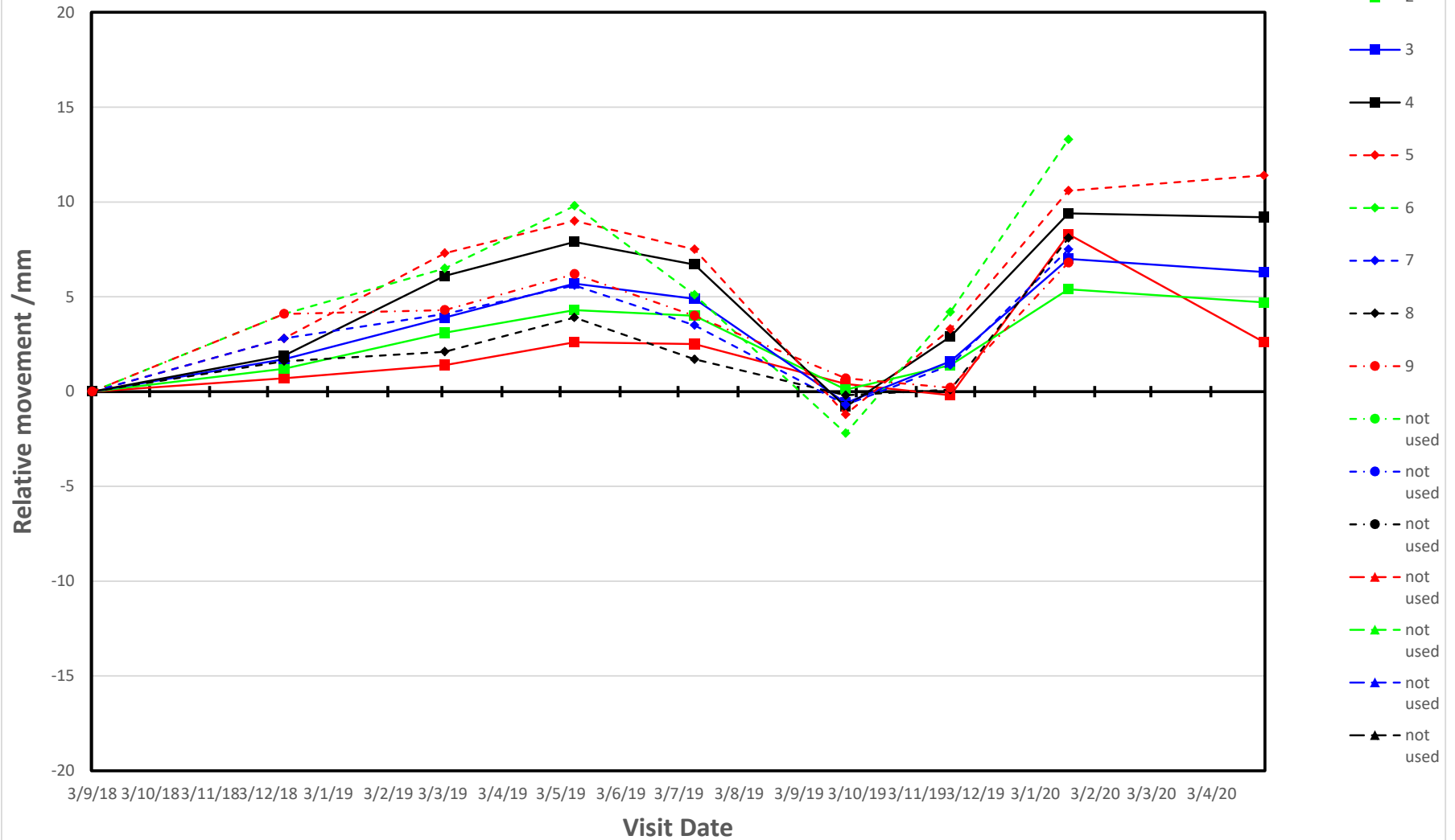
Level Monitoring - Movement relative to datum against Date
