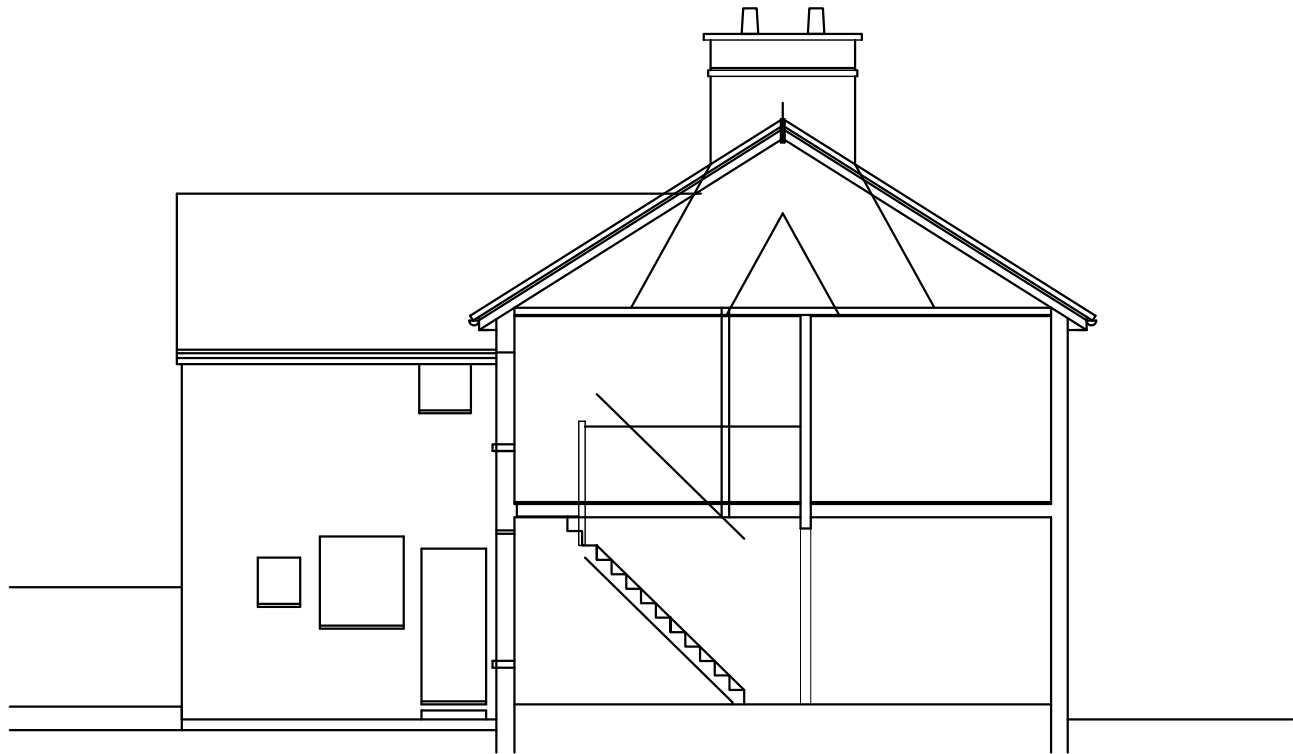
sectional side from No 17 EXISTING
