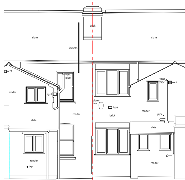
Rear Elevation (E)
