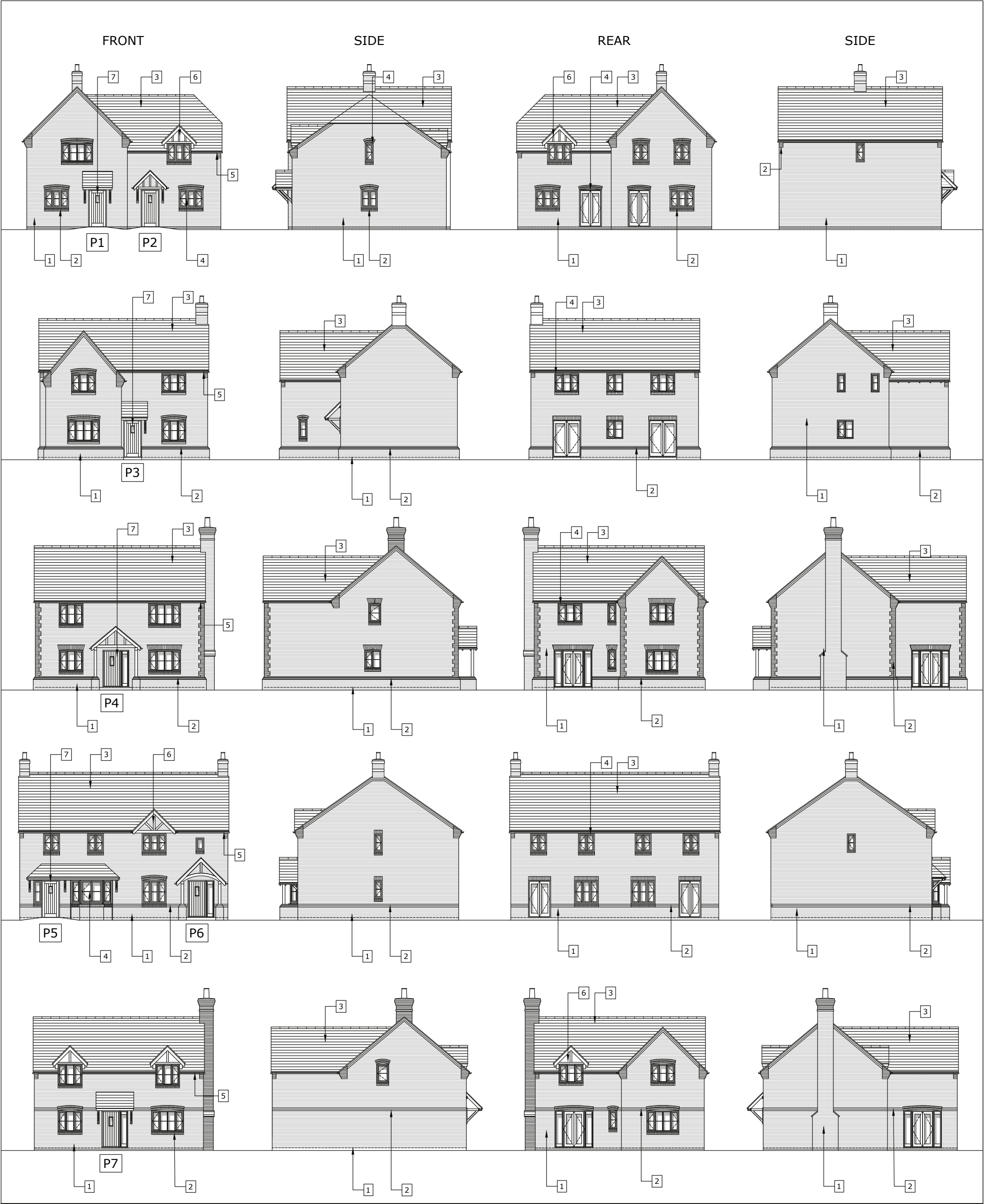
1 - Facing Brickwork
