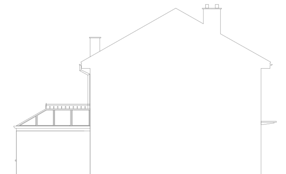
Side Elevation 1:100
