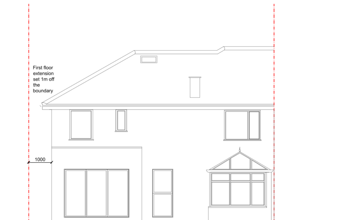
Side Elevation 1:100
