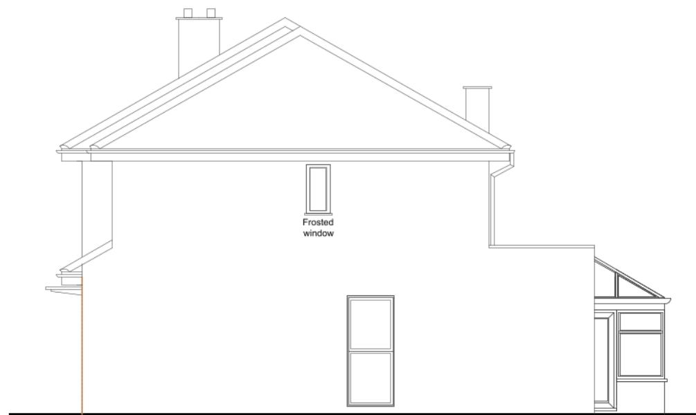
Side Elevation 1:100
