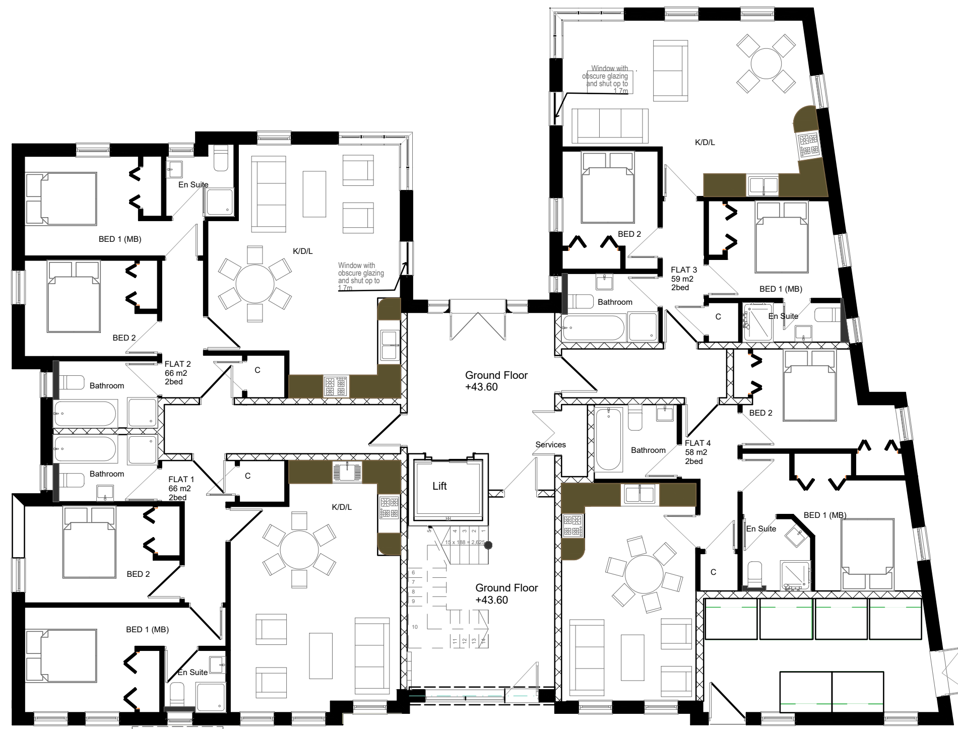
GROUND FLOOR
