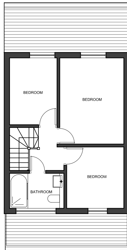
02 - FIRST FLOOR PLAN
