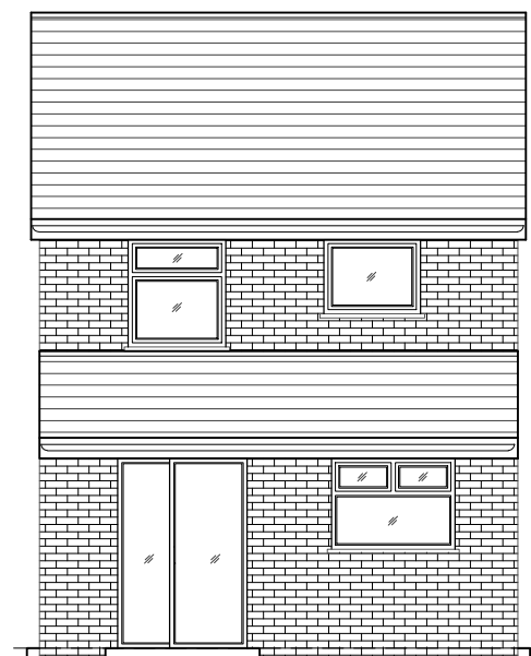
05 - REAR ELEVATION
