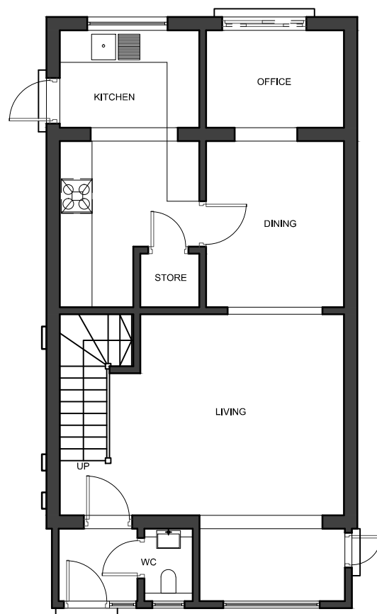
01 - GROUND FLOOR PLAN
