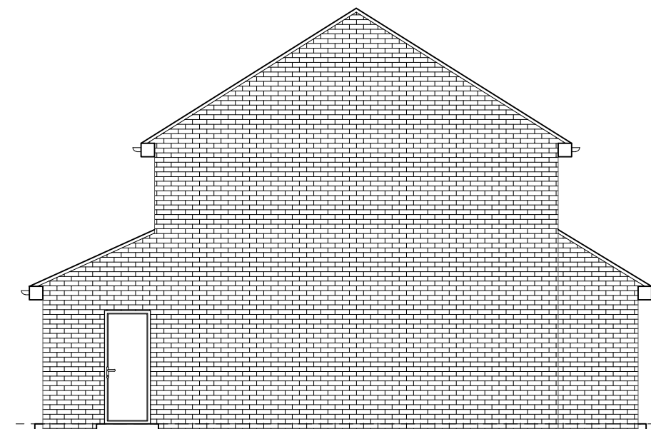
07 - LEFT SIDE ELEVATION
