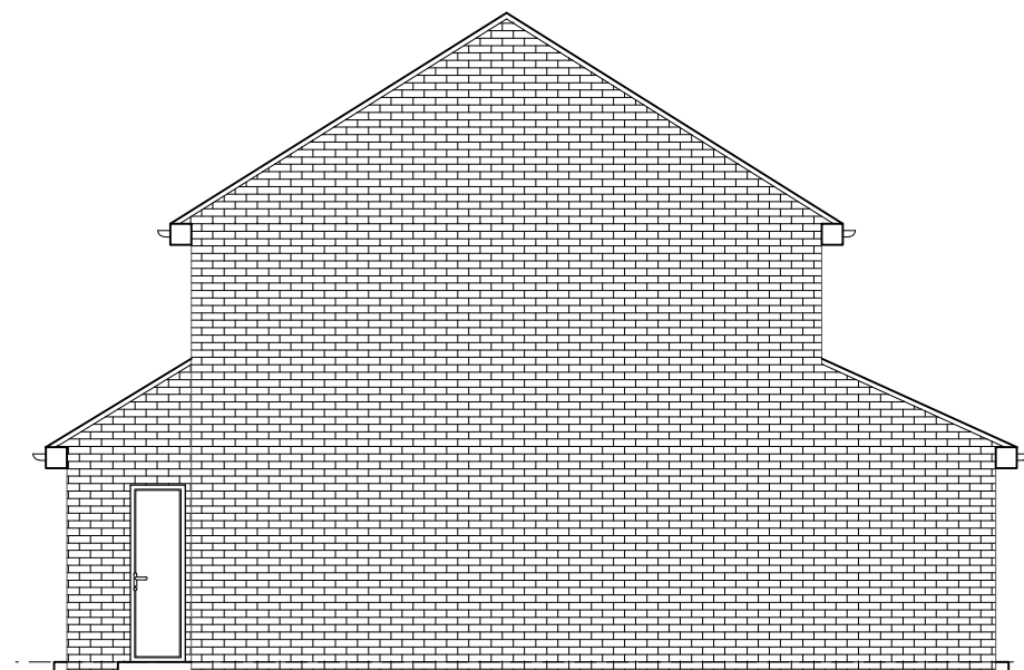
06 - RIGHT SIDE ELEVATION
