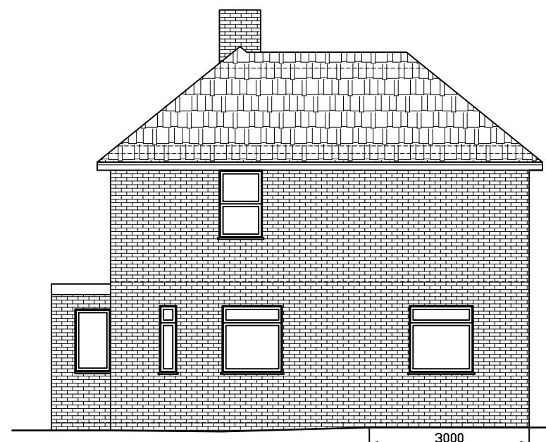
PROPOSED RIGHT SIDE ELEVATION
