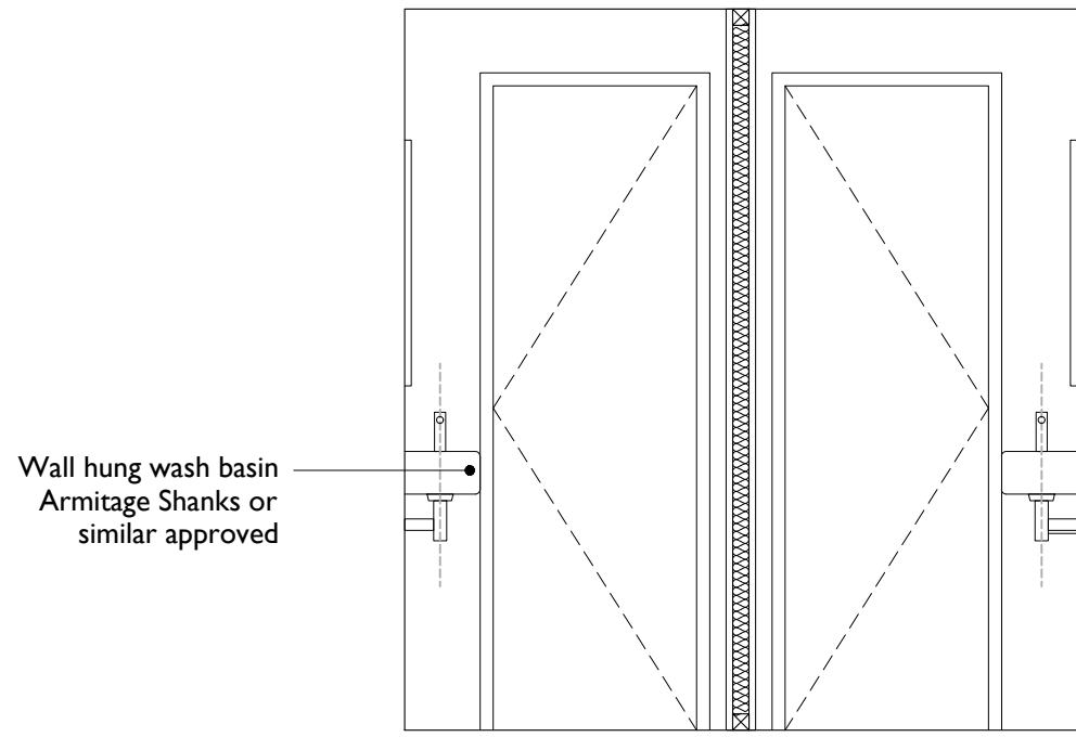
05 Elevation 04
