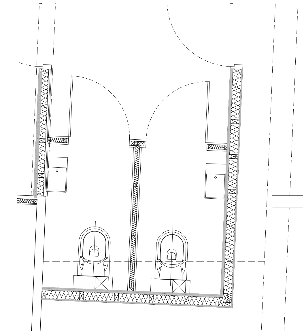
01 First floor plan extract
