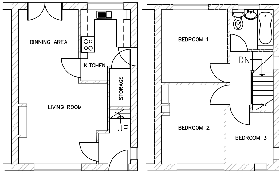
GROUND FLOOR EXISTING
