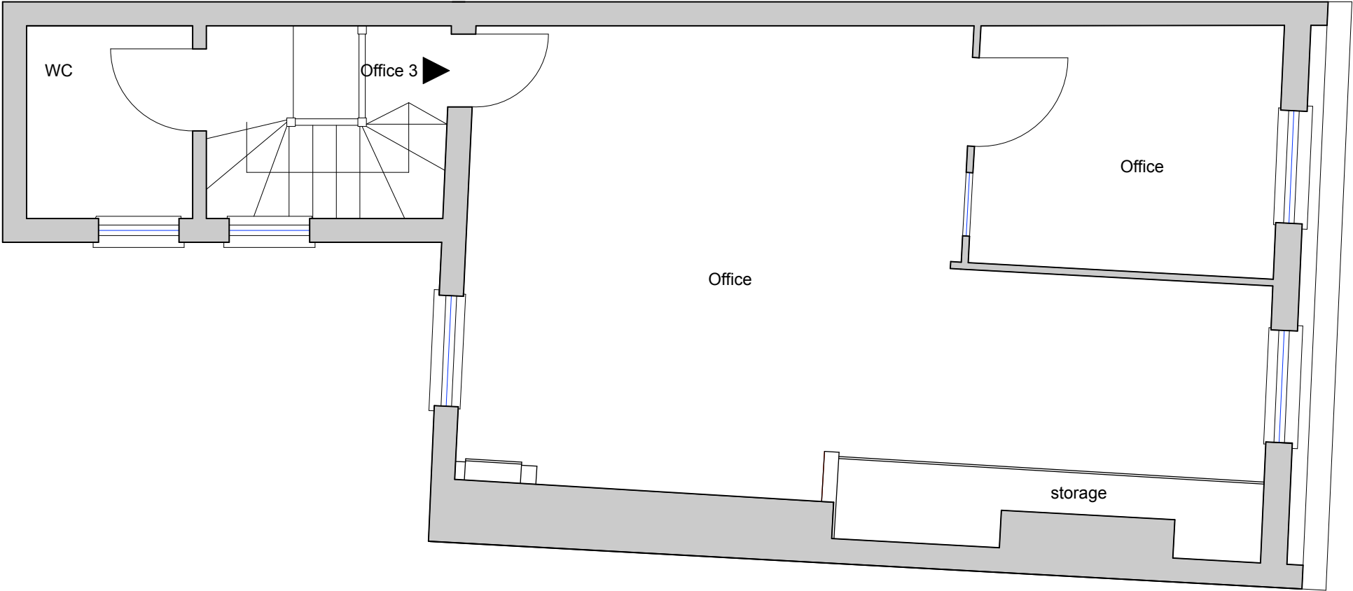
3rd Floor Plan Existing
