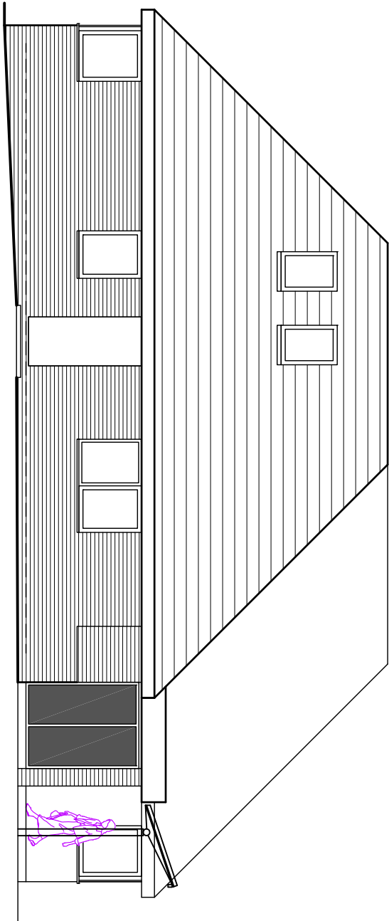
Entrance Elevation (to South)
