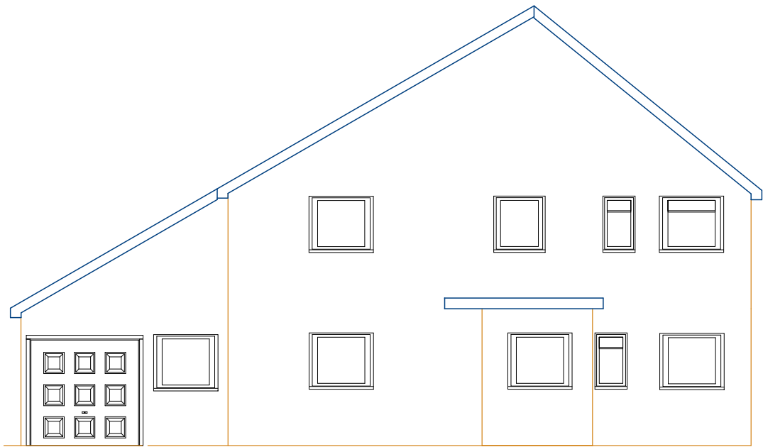
Front Elevation
