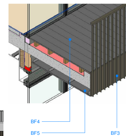
CONCRETE BALCONY
