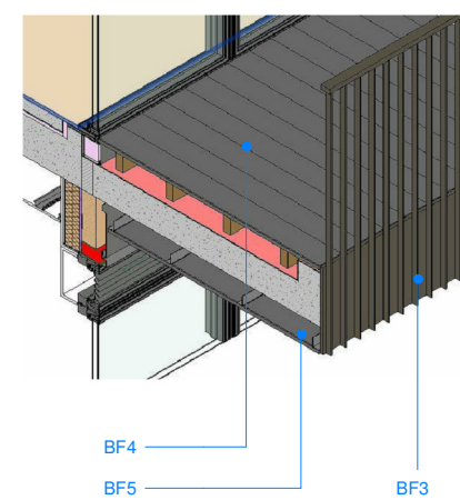
CONCRETE BALCONY
