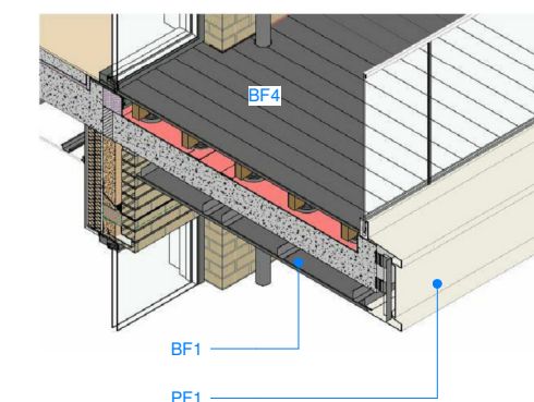
TYPICAL BALCONY
