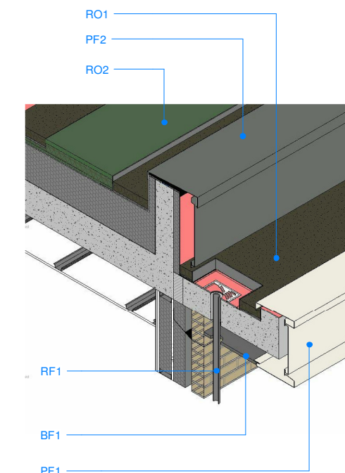
TOPMOST ROOF
