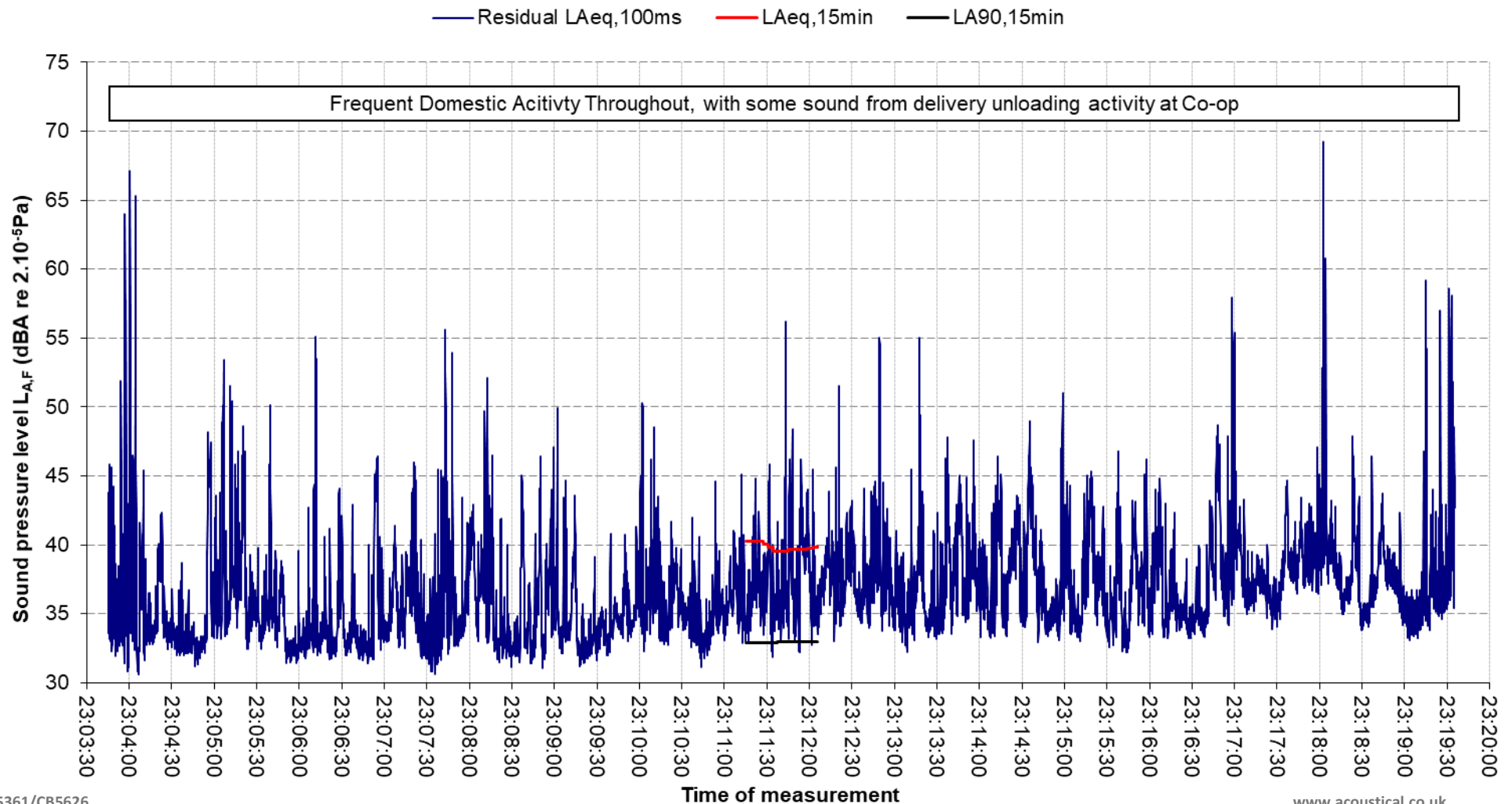
Graph 2 - Existing residual sound level in vicinity of Store Measured 21 st January 2021
