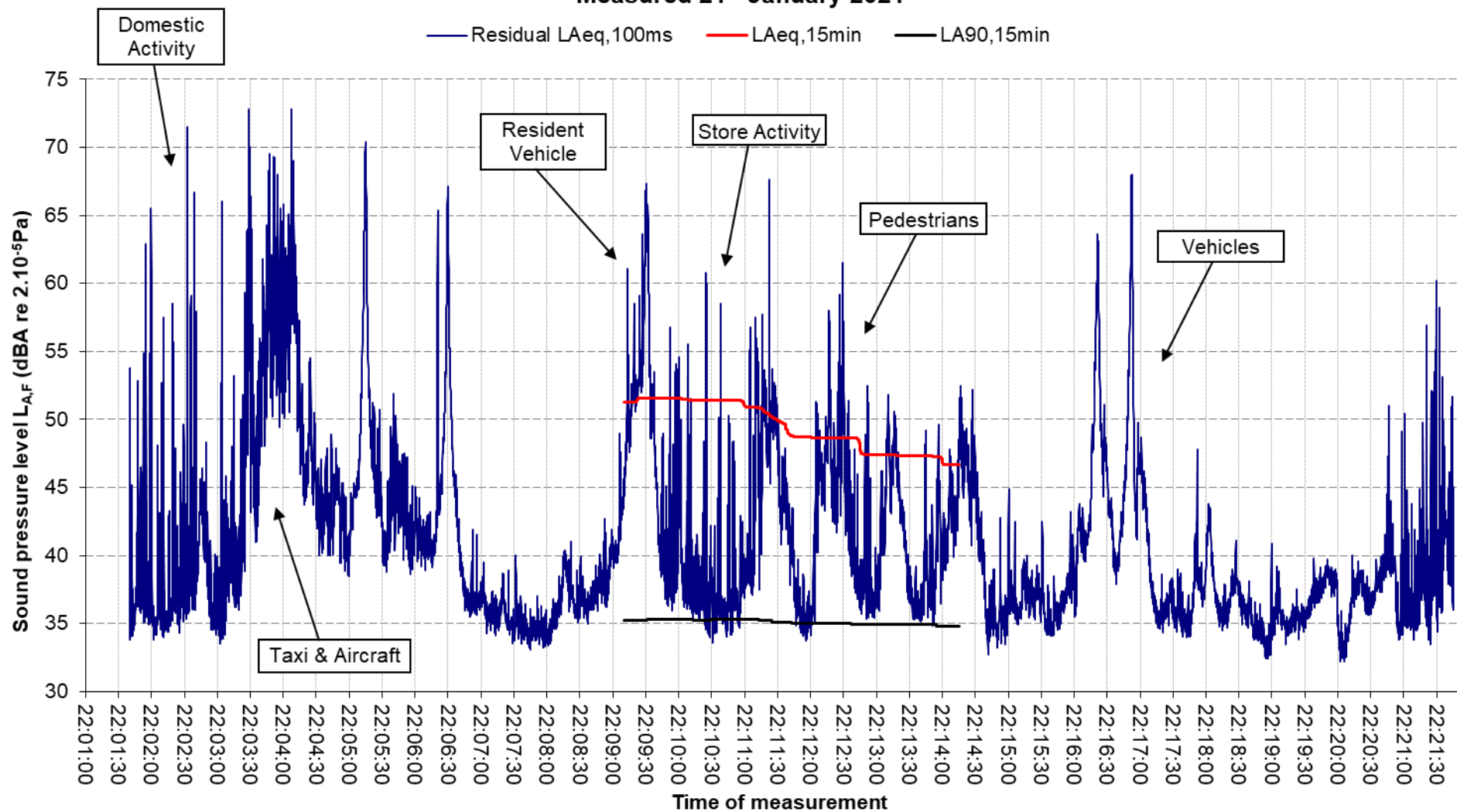
Graph 1 - Existing residual sound level in vicinity of Store Measured 21 st January 2021
