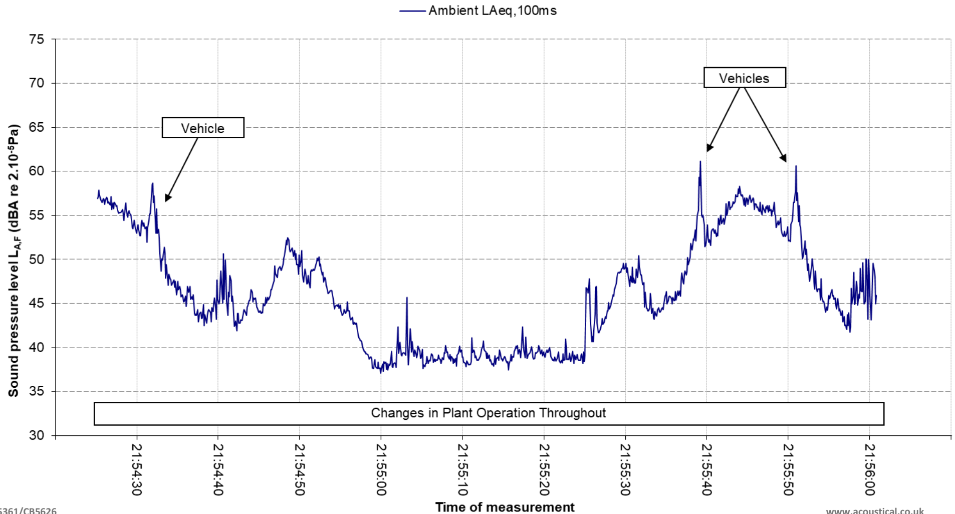
Graph 3 - Existing plant sound level 3 m from plant room louvre Measured 21 st January 2021
