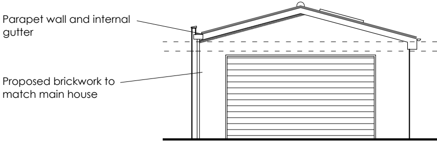
Front elevation 1:100
