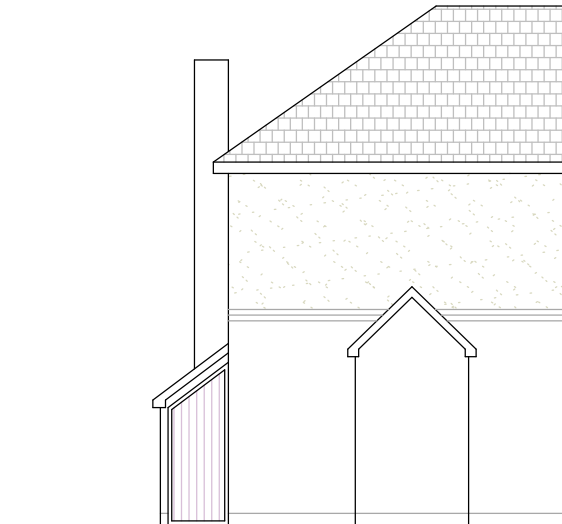
Existing Alternate Side Elevation (Extract)
