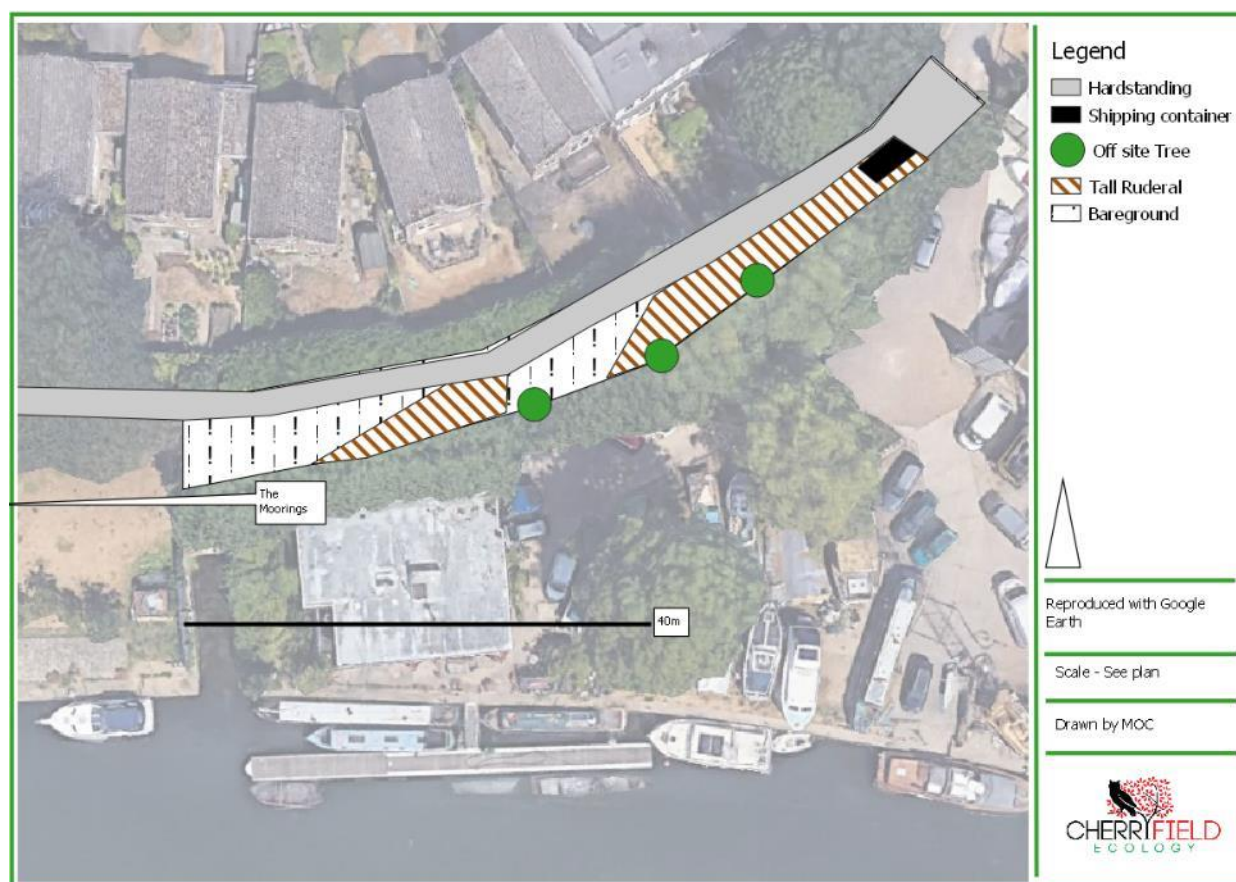
Figure 4: Site Plan
