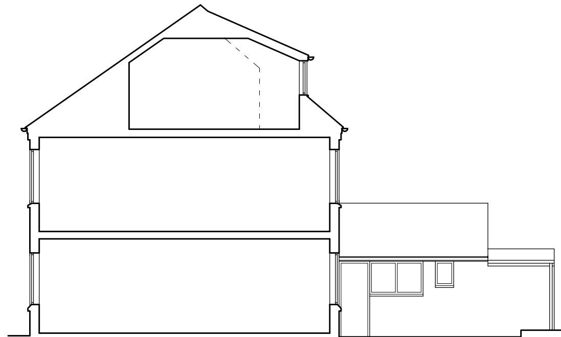
WEST ELEVATION
