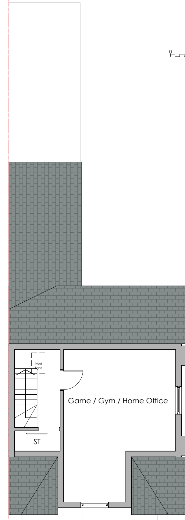
Second Floor
