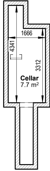
1 EX 00. Cellar floor plan 1 : 100
