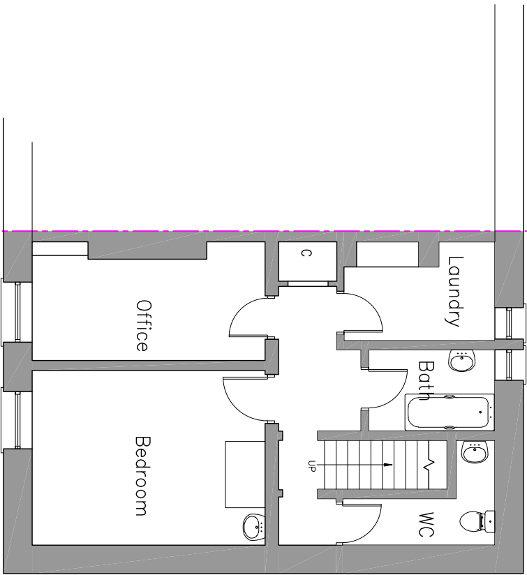
LOWER GROUND FLOOR SCALE 1:100
