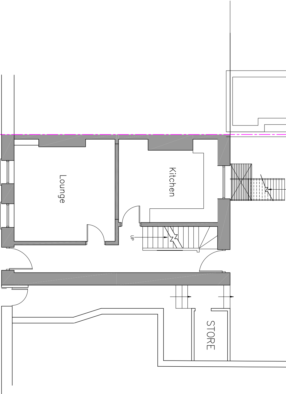
UPPER GROUND FLOOR SCALE 1:100
