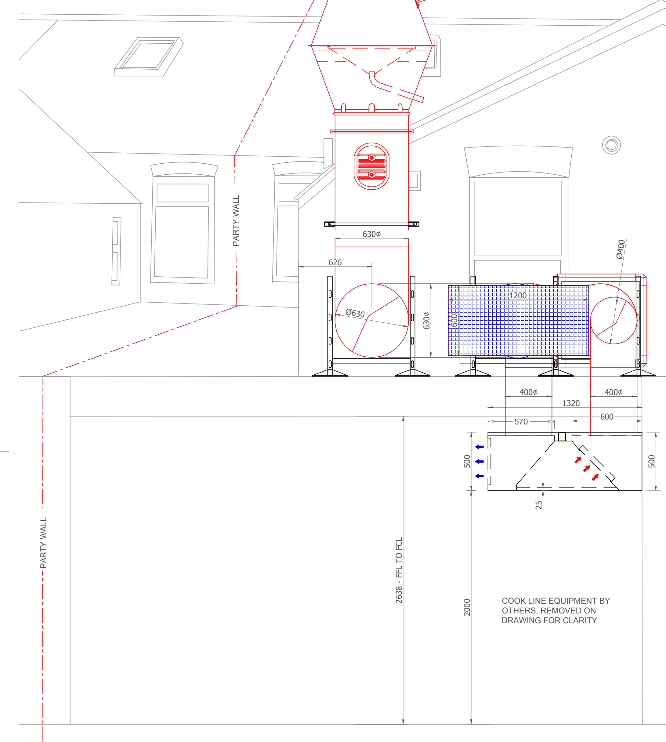
HIGH VELOCITY JET COWL SWEDISH COWL
