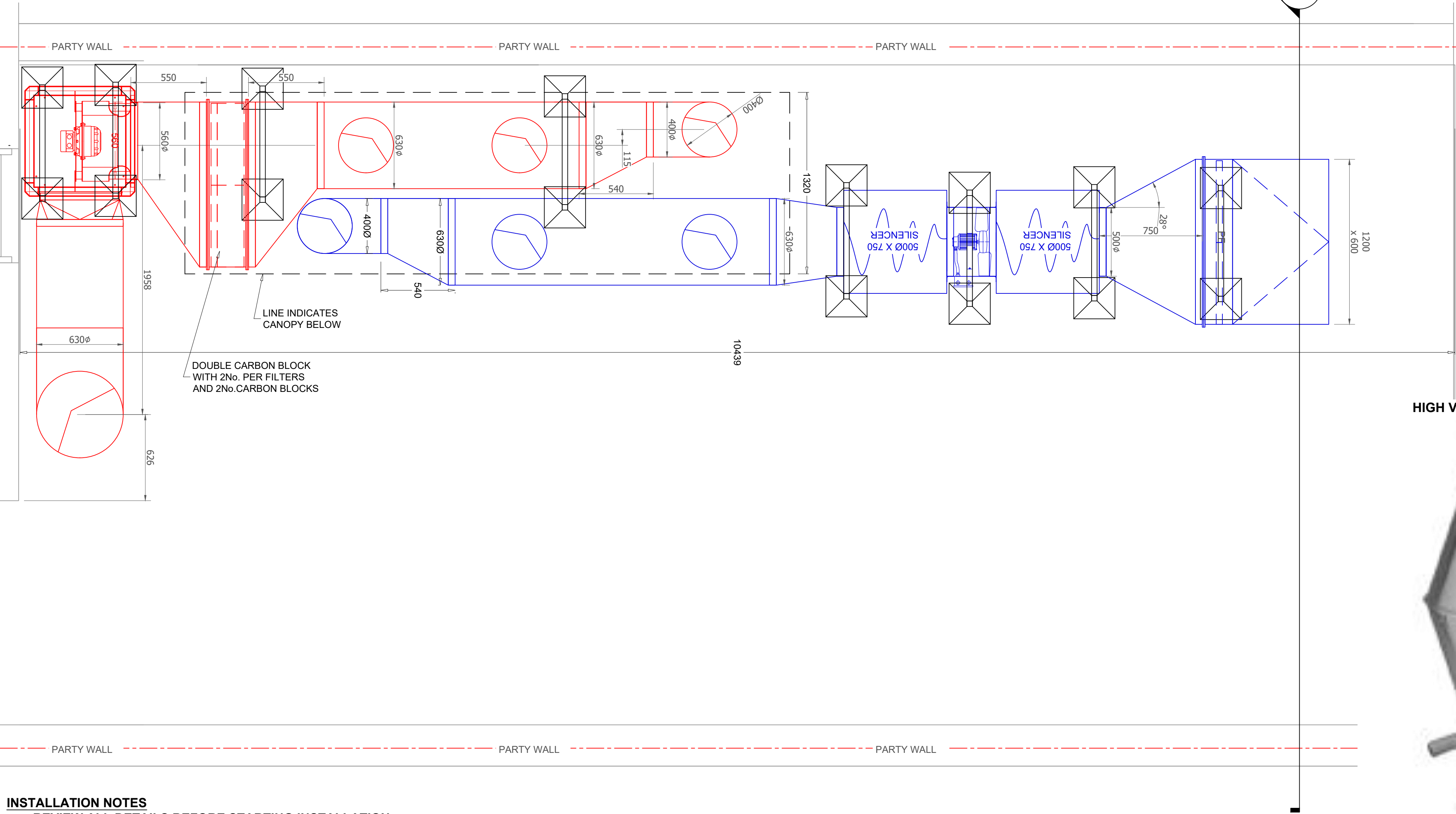
2 PLAN - EXTERNAL VIEW SCALE - 1:20
