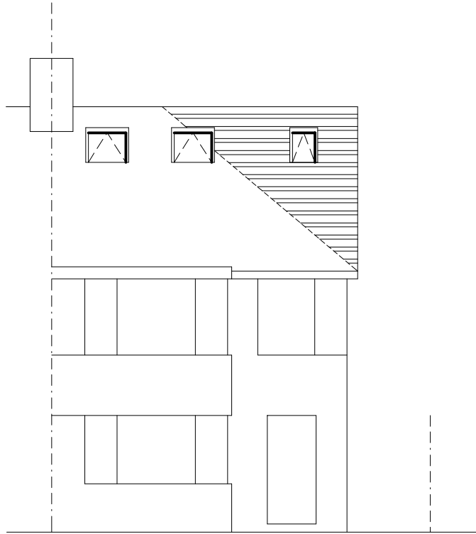
FRONT
