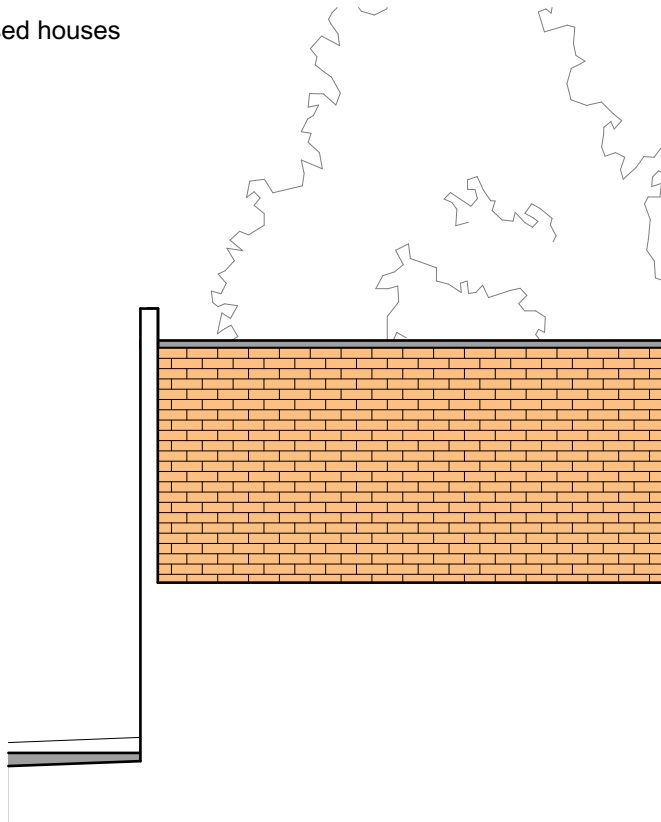
BIN WEST ELEVATION
