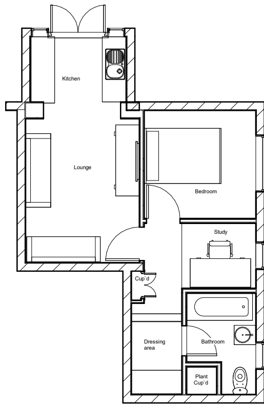
1 Ground floor 1 : 100
