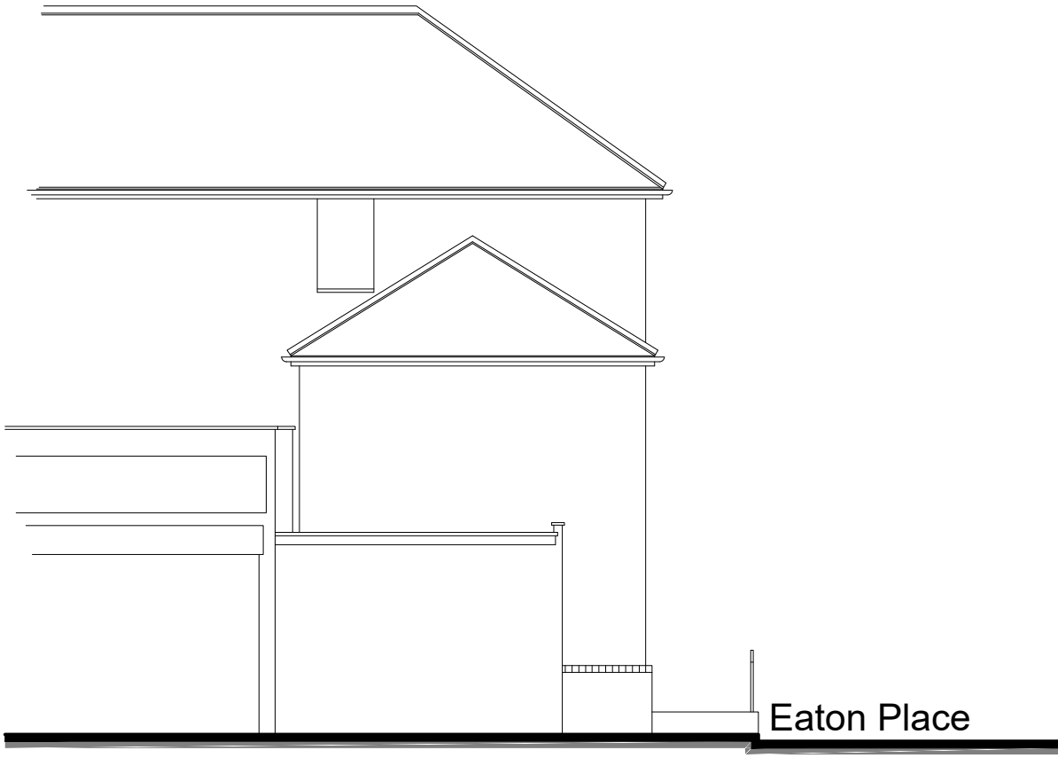
Side Elevation 1:100 scale
