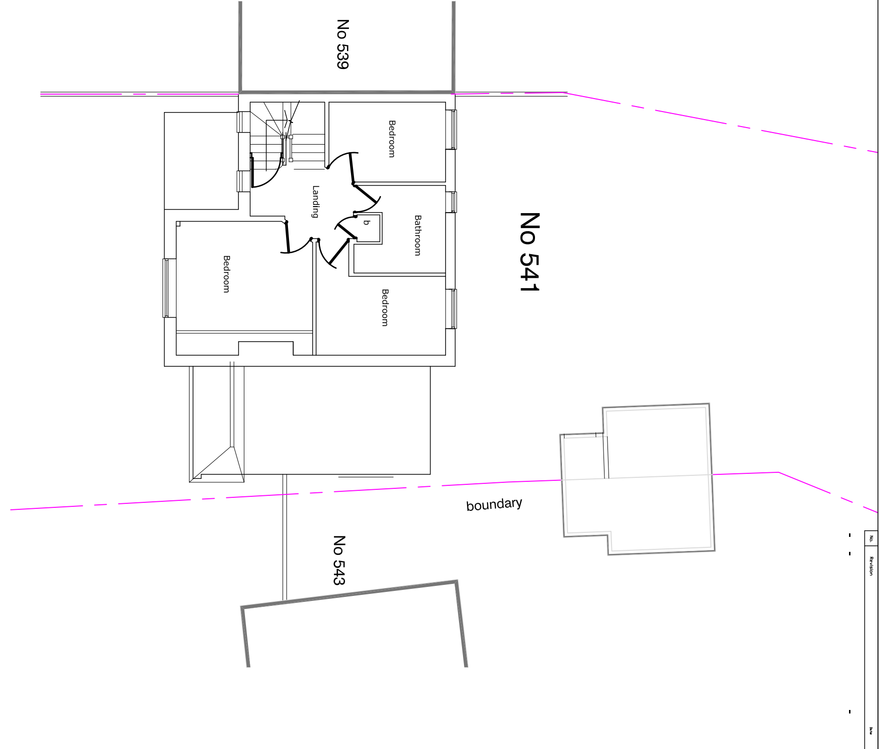
FIRST FLOOR PLAN - Pre-existing
