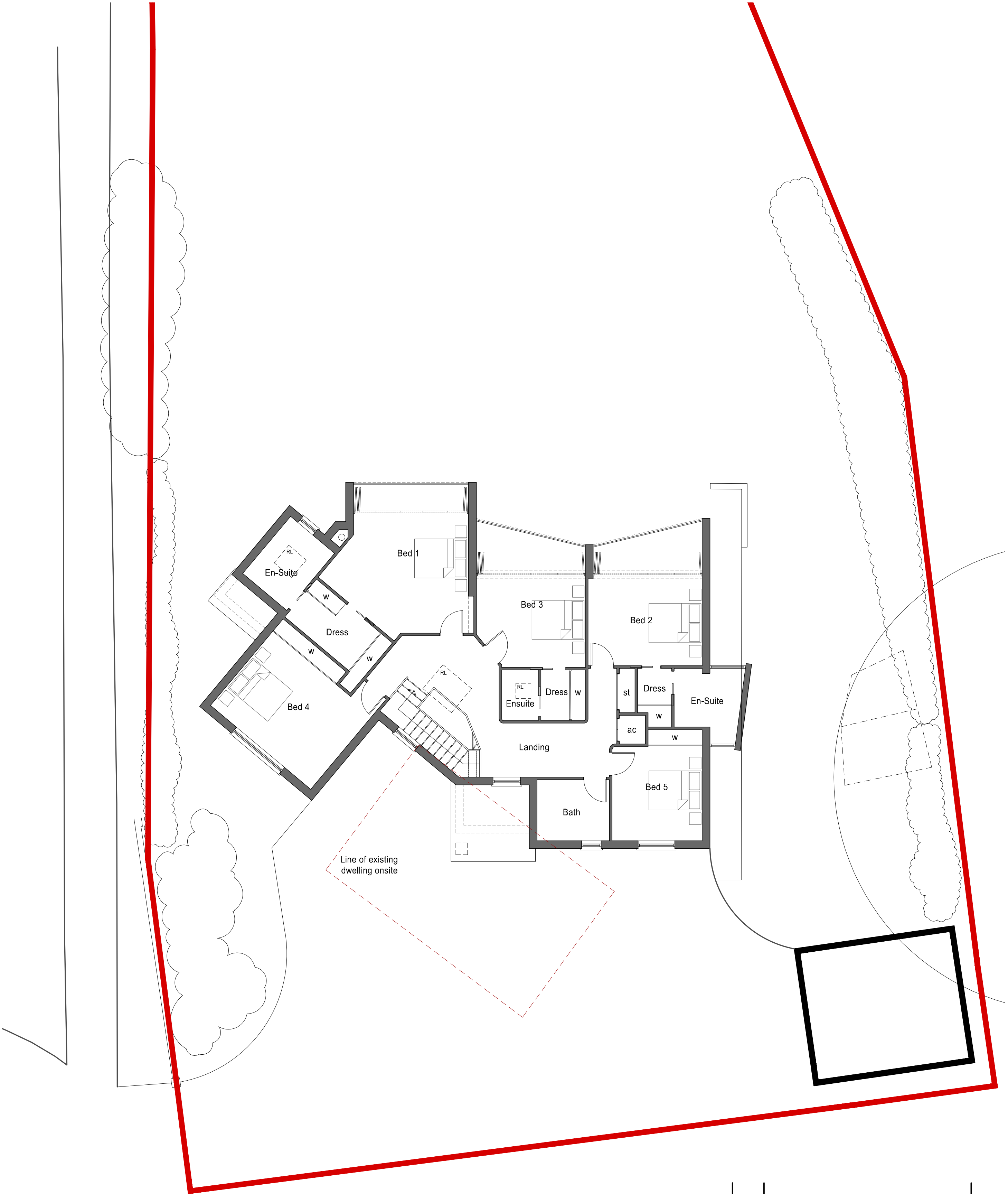
First Floor Plan 1:100 Scale
