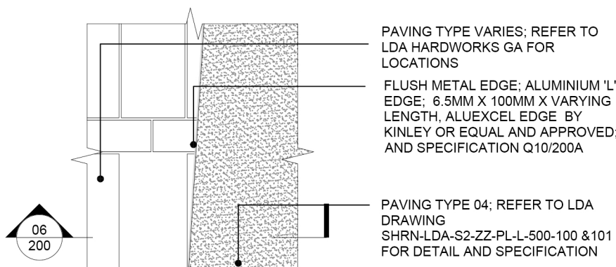
05 TYPICAL DETAIL - FLUSH METAL EDGE INTERFACE TO SAFETY SURFACE 200 PLAN SCALE 1:25
