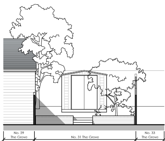
EXISTING REAR GARDEN NORTH-EAST ELEVATION
