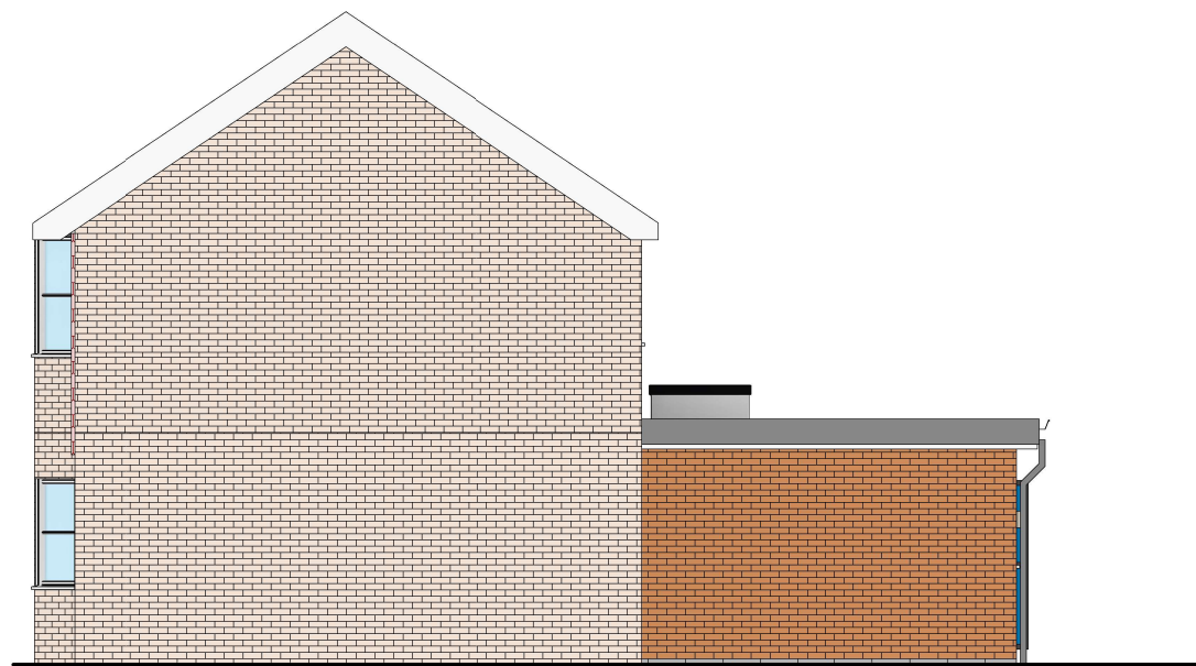
Proposed Right View 1 : 100
