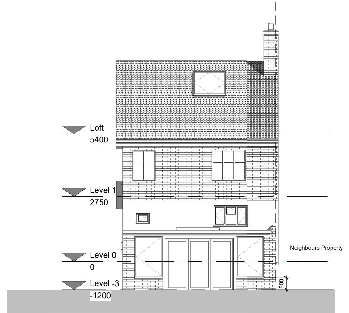
2 Rear elevation - Proposed 1 : 100
