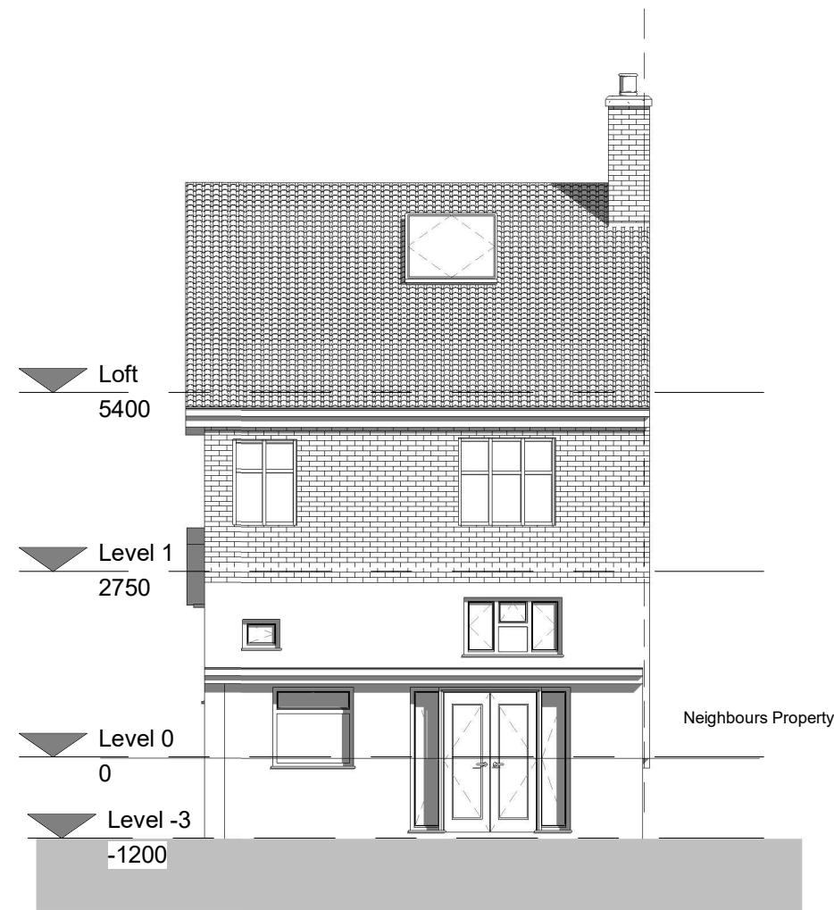
1 Rear elevation - Existing 1 : 100
