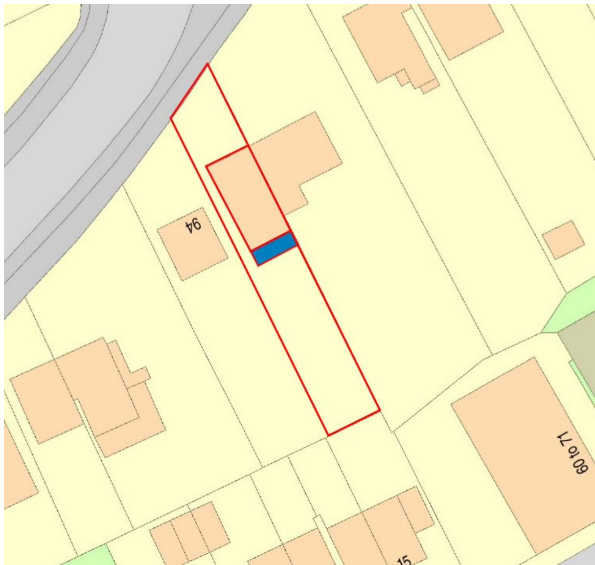
1 00 - Block Plan 1 : 500
