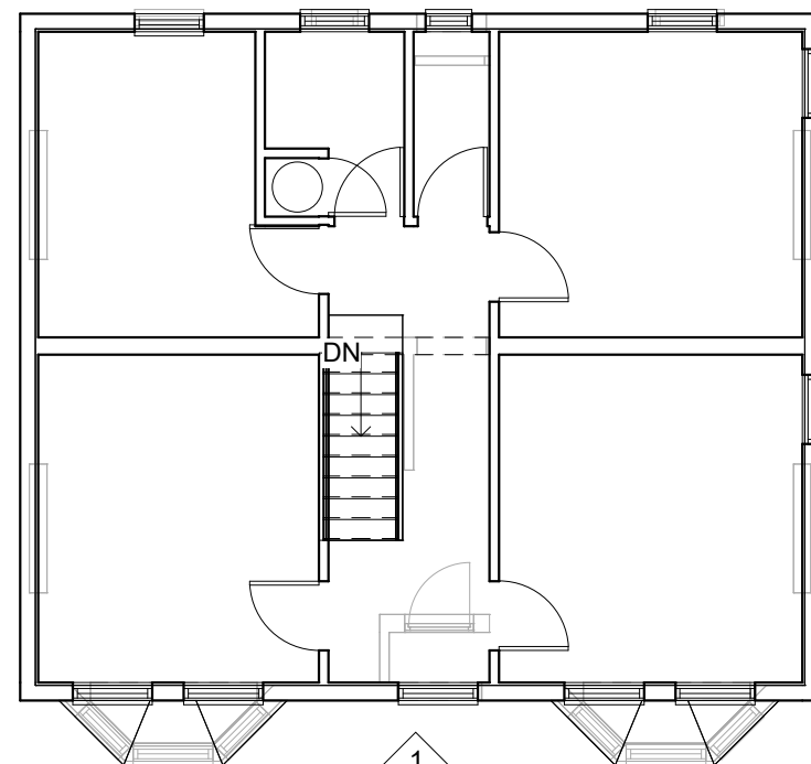
4 Exist First floor 1 : 100
