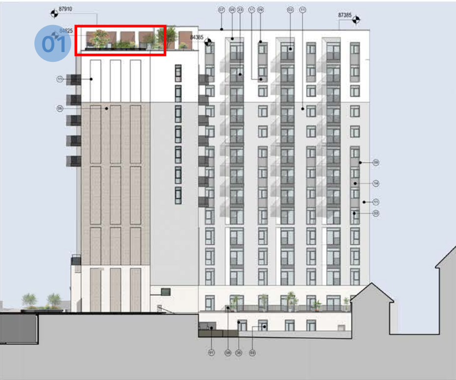
1 Block F - South Elevation 1: 250
