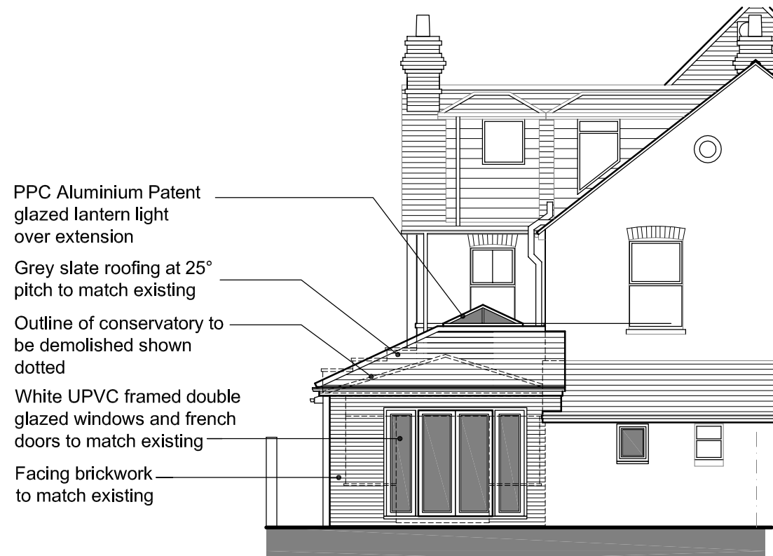
NORTH ELEVATION
