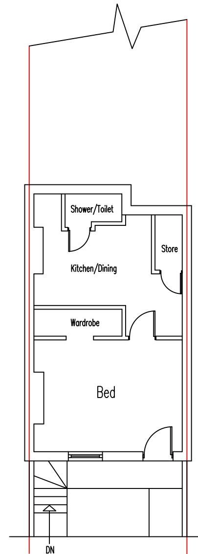
Existing Lower Ground Floor
